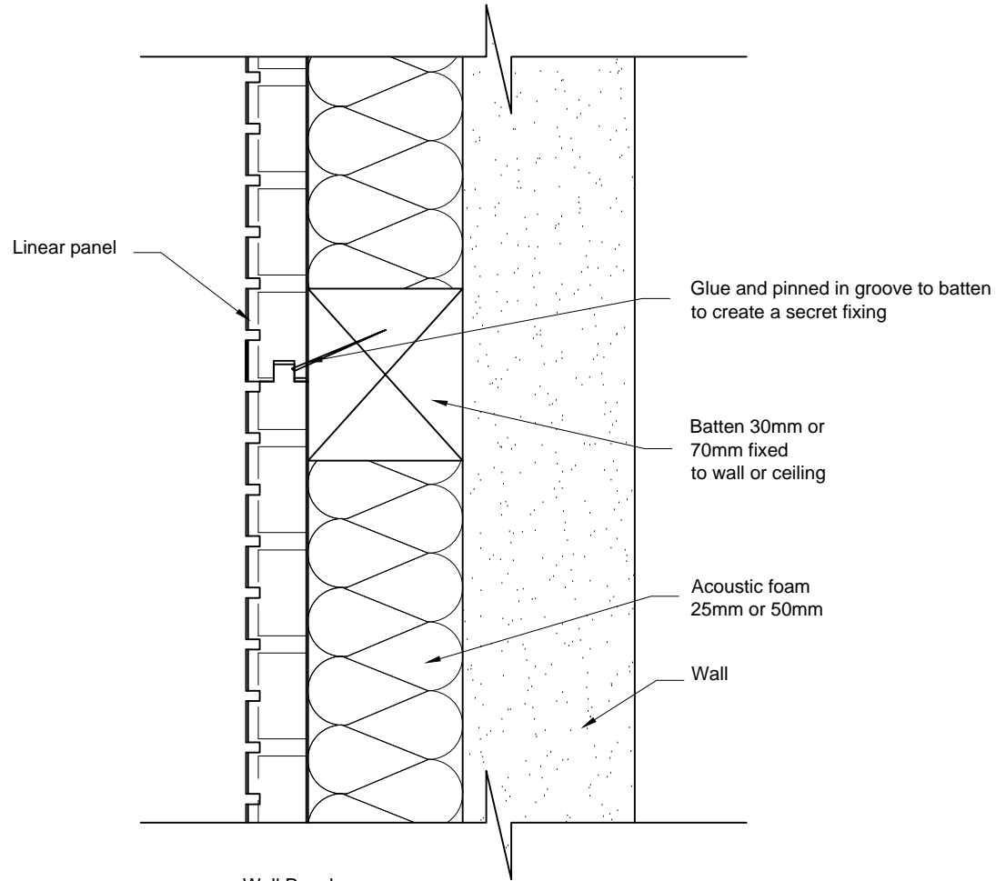
Wall Panel Scale 1:2
